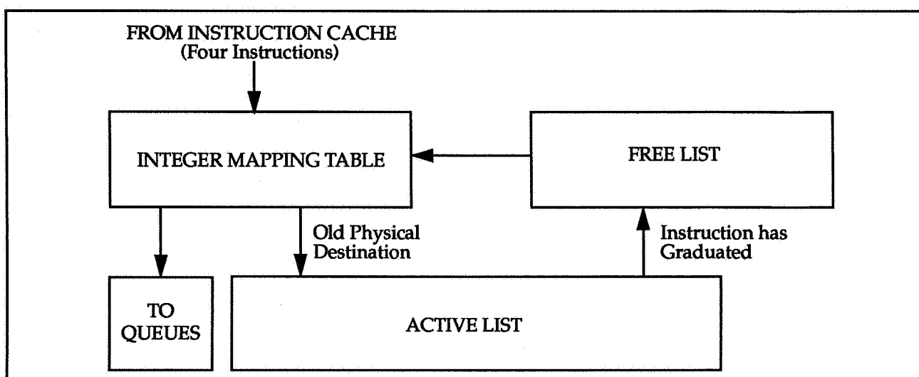
Figure 6 Integer Instruction Mapping Scheme Block Diagram
