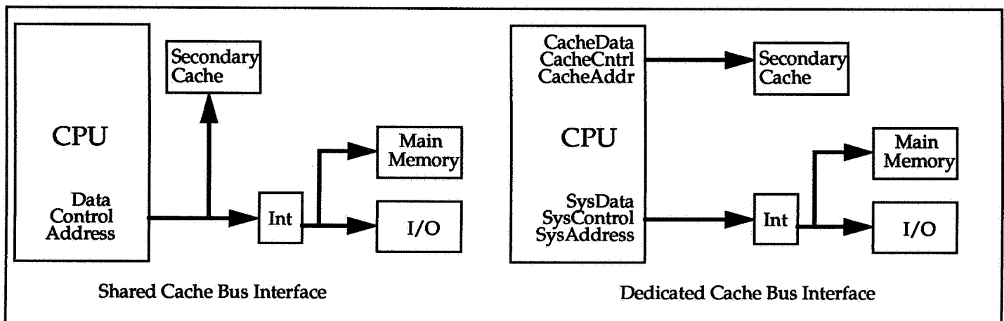
Figure 3 Dedicated Secondary Cache Bus Interface
